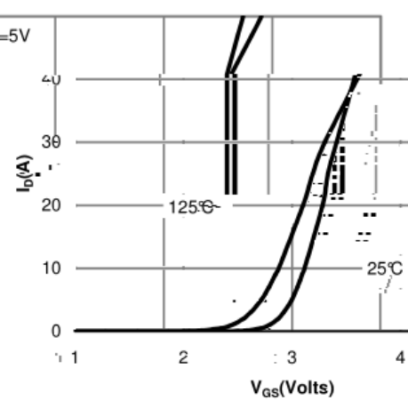
Figure 2: Transfer Characteristics
